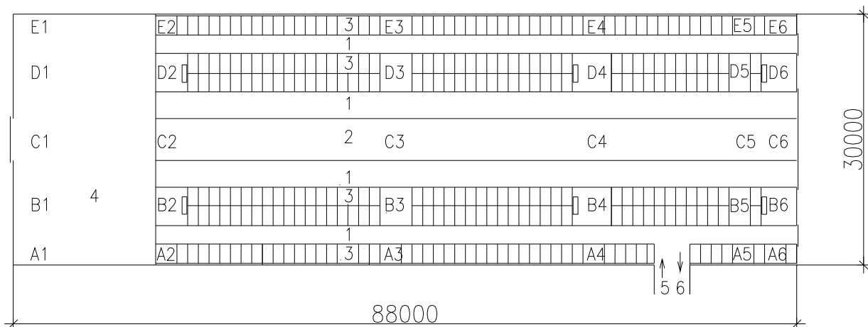
Figure 1. The layout of cowshed. 1 – walking area, 2 - feeding alley, 3 – cubicles, 4 - feed storage and service area, 5 – entrance to milking parlour, 6 – exit from milking parlour, A1...E6 - the measurement points
